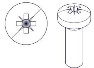
M5 x 16 (PZ-2)
